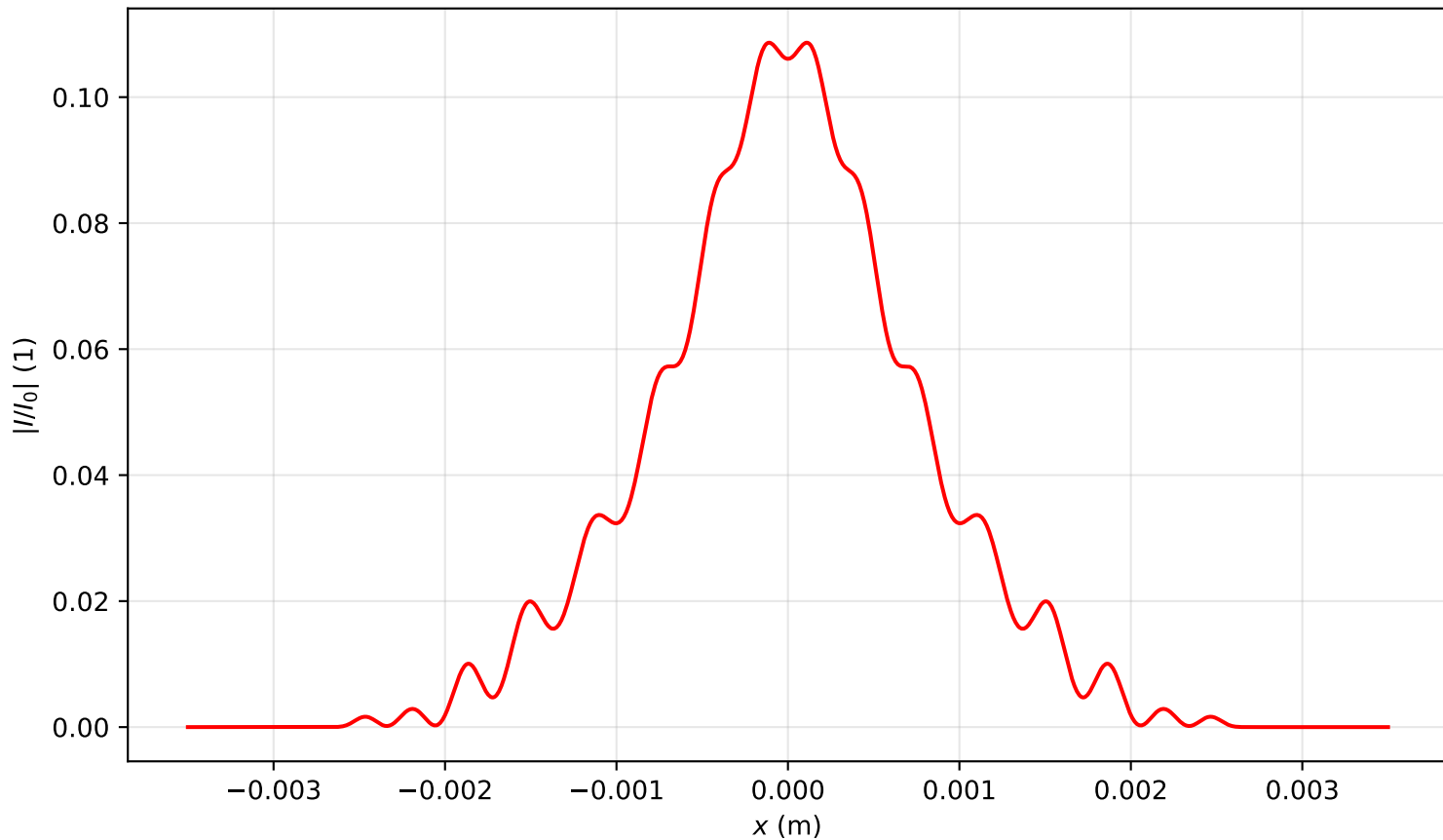
Intensity profile I(x, y = 0, z = 2.388)/I_0 , P_{in}=2.0P_{cr} , artificial time
